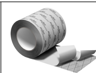
Abb. 2: Difutape 150 mm
