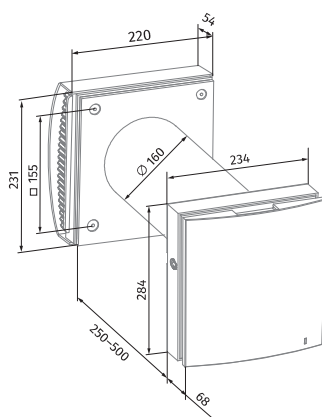
VENTO Expert A50-1 S10 Pro
